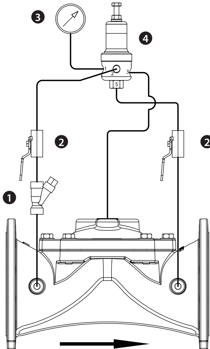
Pressure Sustaining Control Valve - 2 Way
