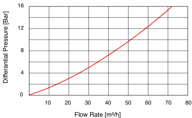
S-050 / S-050-C AUTOMATIC AIR RELEASE FLOW RATE
