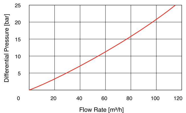
S-052 AUTOMATIC AIR RELEASE FLOW RATE
