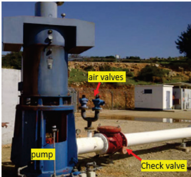
Figure 2. General arrangement at pump station PS-1
