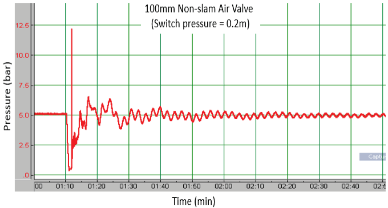
Figure 6. Variation in measured pressure at critical air valve location with non-slam air valve
