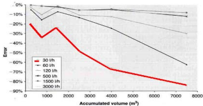
Figure 3: Evolution of the metering Error obtained from a sample of volumetric meters (1/2") (Arregui et. 2006, p.28)
