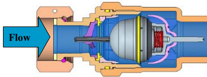
Figure 9: UFR opens: downstream pressure equals that of upstream
