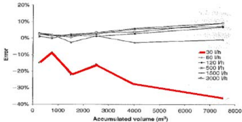
Figure 2: Multi-jet error (nominal flow 1.5 m 3 /hr) on accumulated volume (Arregui et. 2006, p.21)
