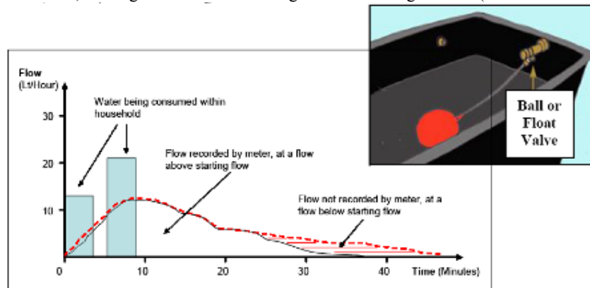
Figure 4: The effect of a roof tank on meter under-registration (Rizzo and S. John, 2006)
