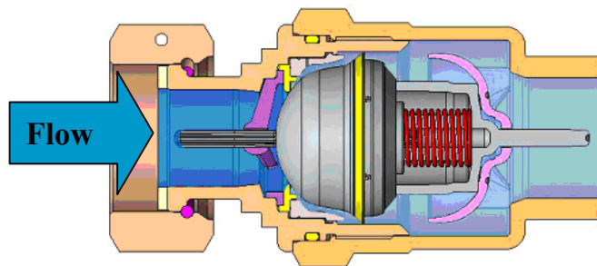
Figure 8: UFR closed: downstream pressure decreases because of leakage
