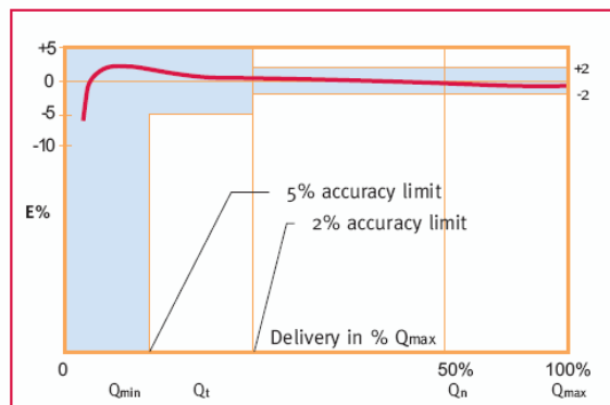
Figure 1: Error curve of a water meter
