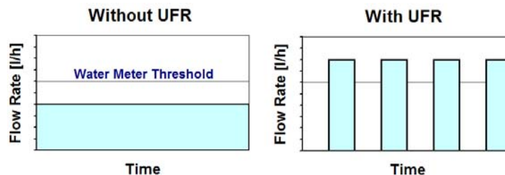
Figure 7: UFR – Principle of Operation
