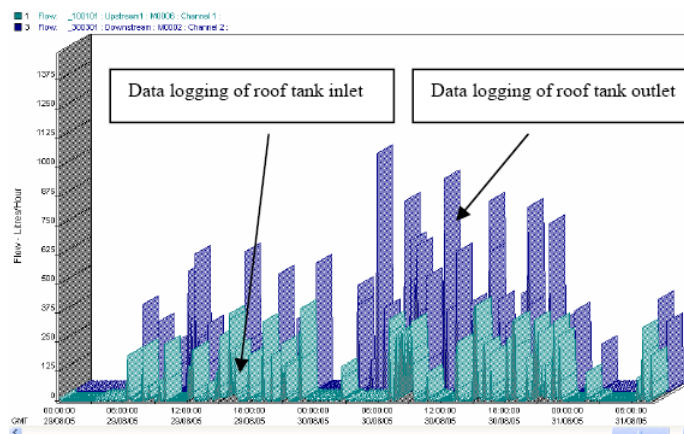
Figure 5: Data logging of water meters at roof tank inlet and outlet (Rizzo and S. John, 2006)
